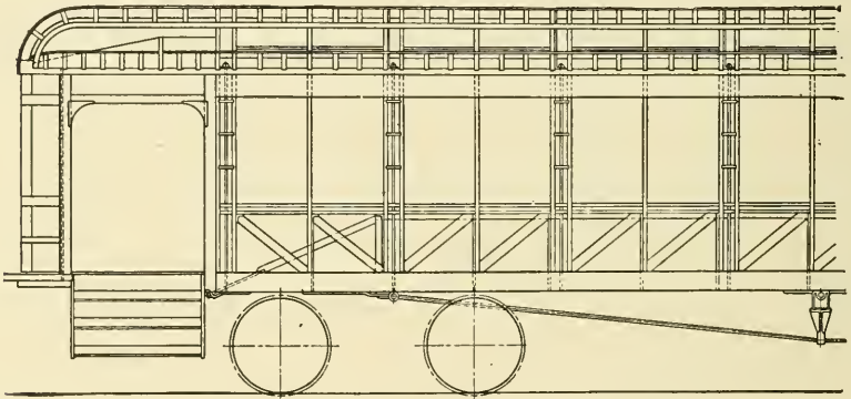
Fig. 5. Side View of Car Framing
